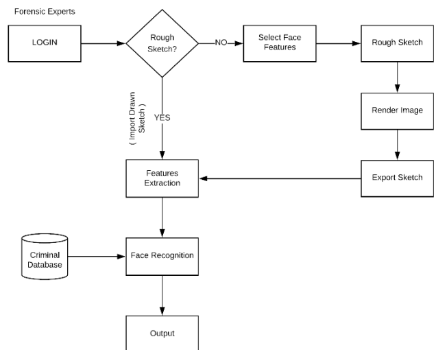
Fig. 6. System Flow of the application
